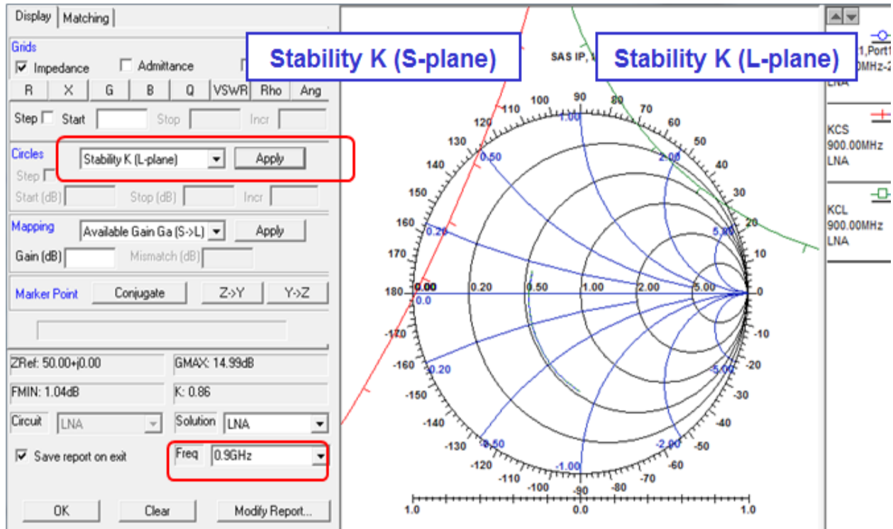
Figure 1-2 Red curve is Stability K (S-plane) and green is Stability K (L-plane)
